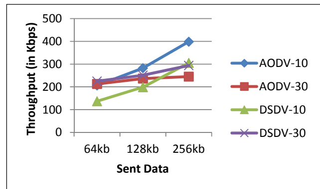
Figure 4.3 Throughput for Scenario 1,2 and 3
