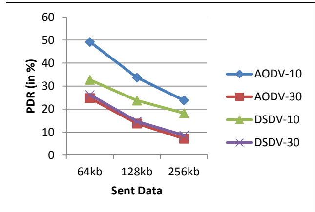
Figure 4.1 Packet Delivery Ratio for Scenario 1,2 and 3
