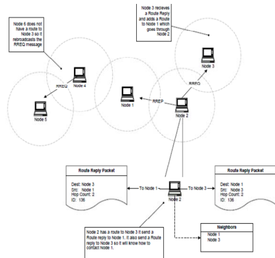
Figure 3.1.: Working of AODV routing protocol
